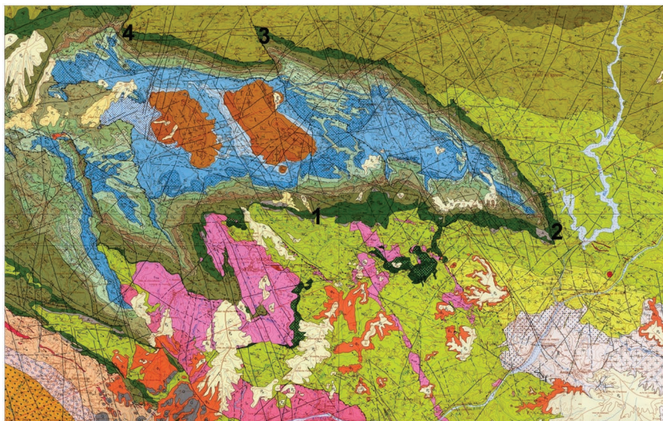
Figure 8. The Mação territory in geological and topographical map showing the hillfort “system”.
